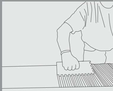
Apply adhesive onto the back of the slab with a 3mm trowel in one direction only.
