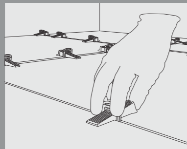
Complete the laying of the slab with a suitable sealant while keeping a 3mm joint through spacers. The special device of pulling over the slabs can be used for easy laying and spacing.
