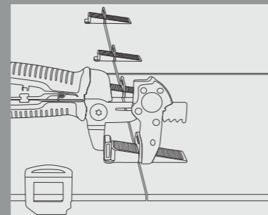
Level the wedges at each linear meter of the slab.
