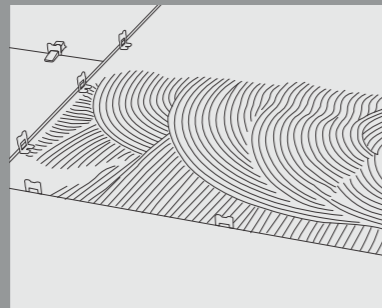
Apply adhesive onto the floor substrate at the same time while applying on the slab with a 15mm U-notch or 19mm V-notch trowel in the same direction as the slabs.
